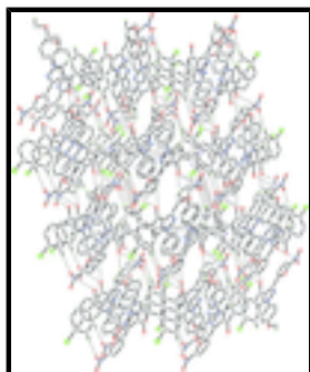
Fig. 2. The crystal structure of (I), viewed along the c axis, showing the three-dimensional extended network. Hydrogen atoms not involved in intermolecular interactions (dashed lines) have been omitted for clarity.
